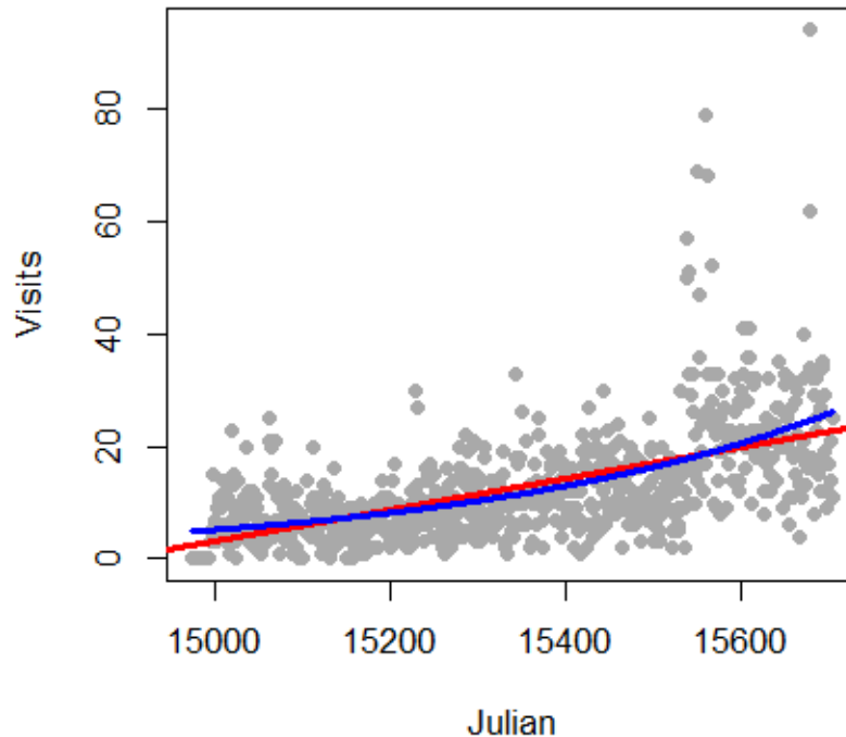
Data with fitted Poisson regression line.
