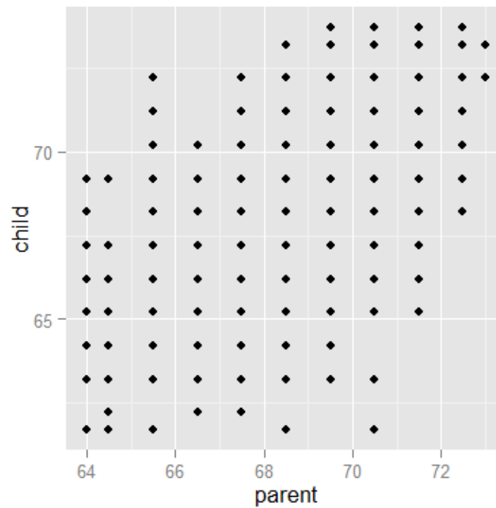
Plot of parent and child heights.
