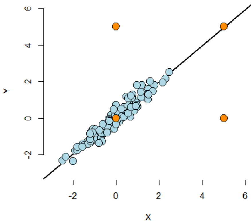
Plot of simulated data with four different kinds of highlighted orange points.
