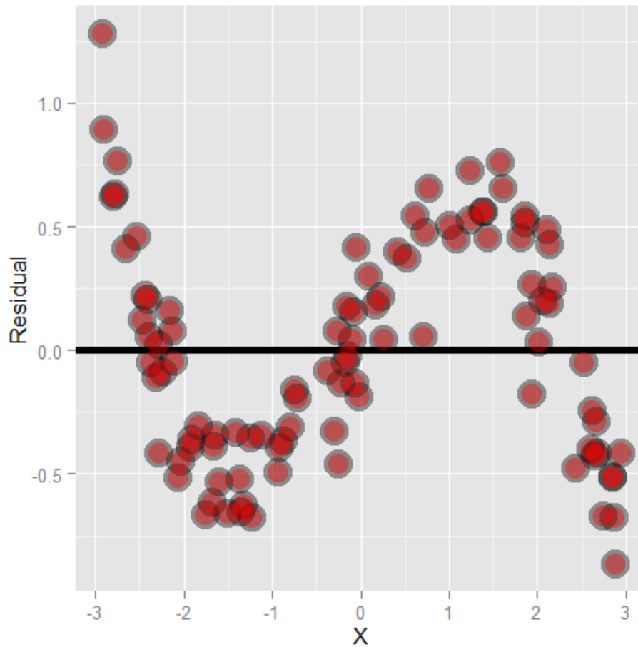
Plot of residuals versus X
