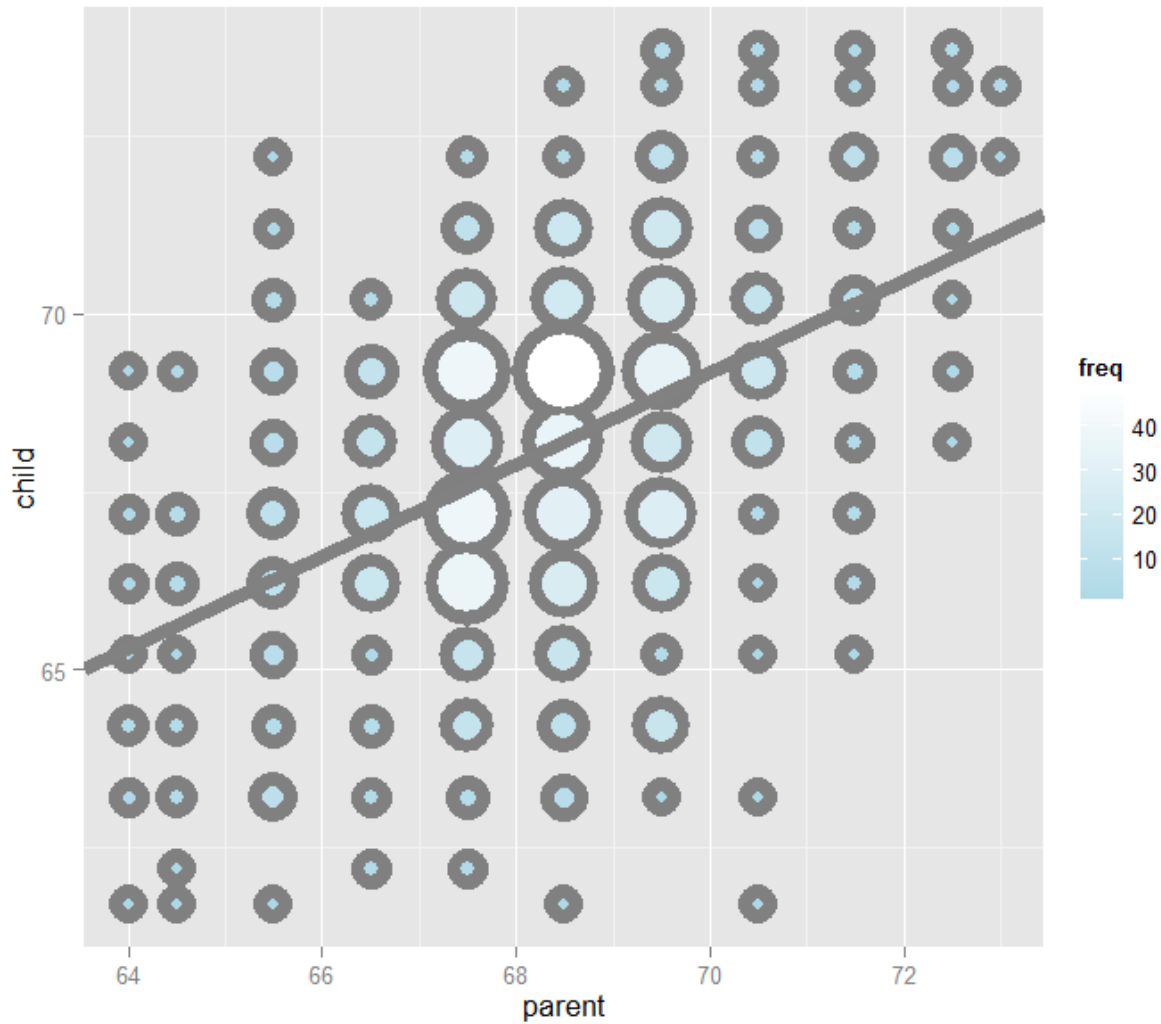
Data with the best fitting line.
