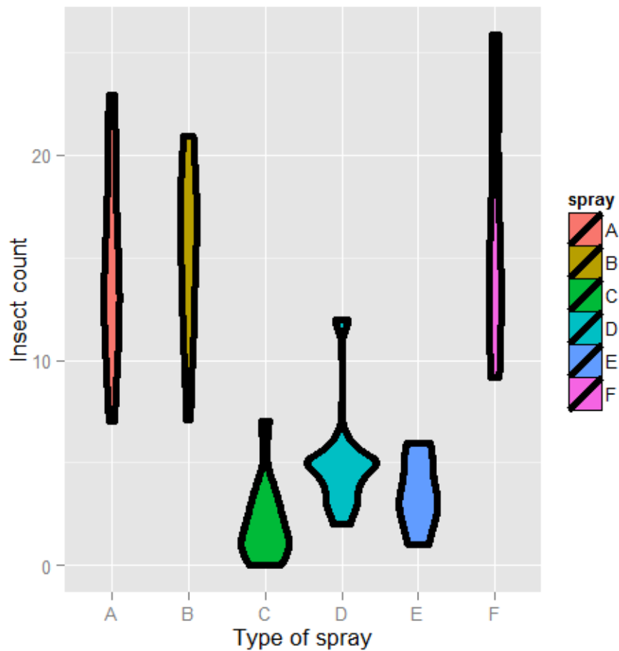
Insect spray dataset
