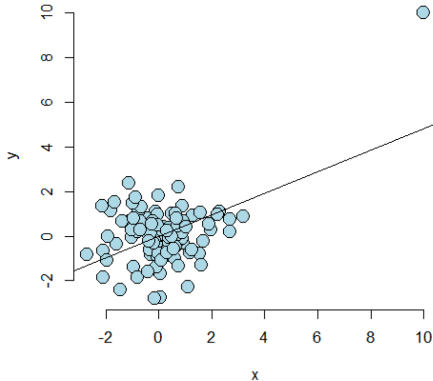
Image for first simulation.
