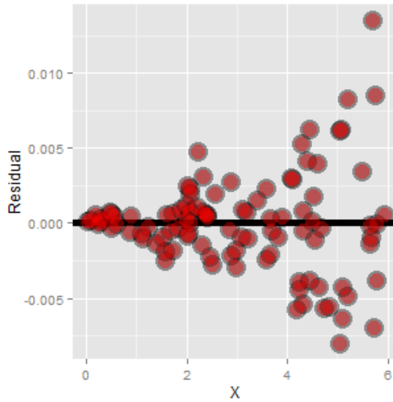
Residuals versus X.
