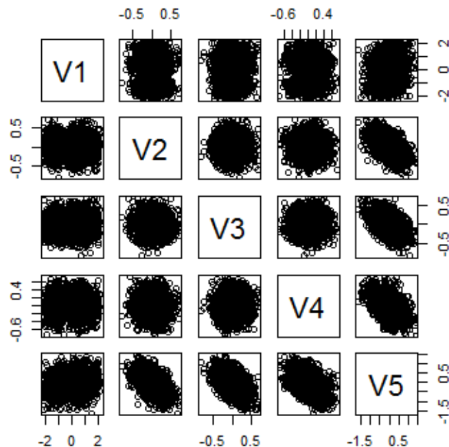
Scatterplot matrix from the Stefanski data.
