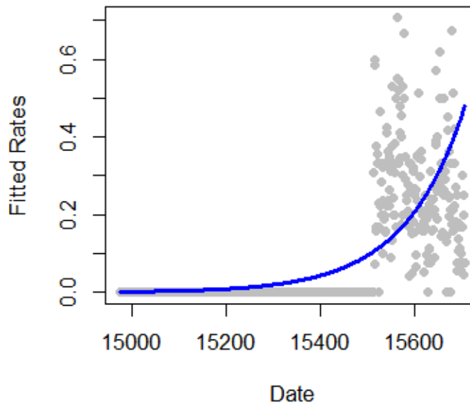
Plot of the fitted rates.
