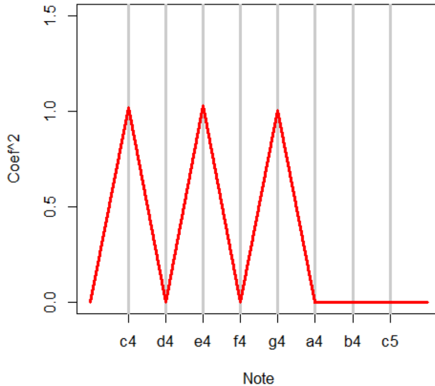
Plot of the fitted coefficients.
