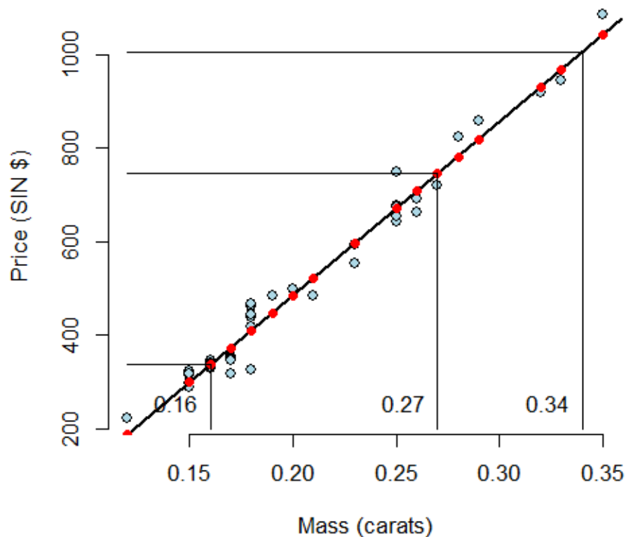
Illustrating prediction with regression.
