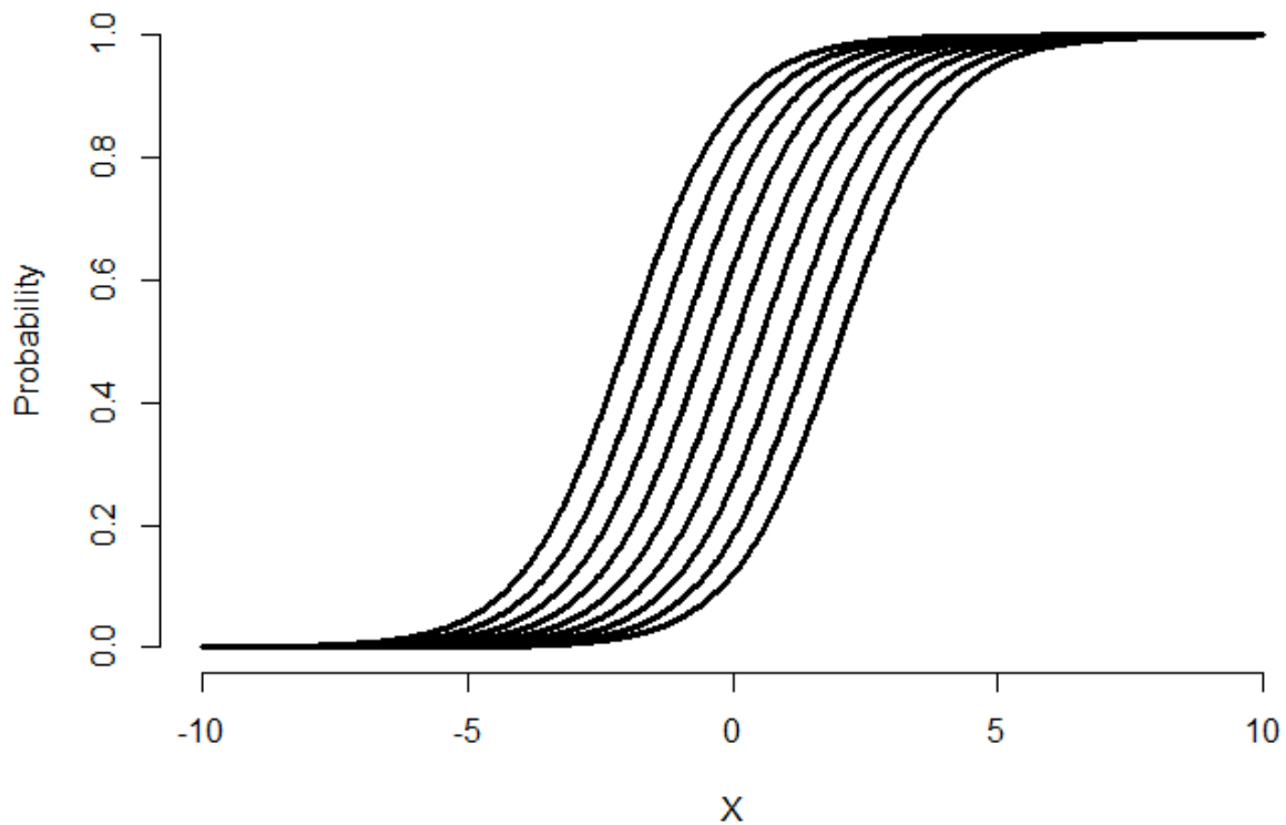
Plot of logistic curves for varying intercepts.
