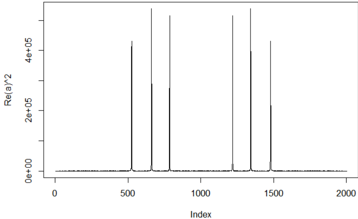
Fit of the FFT to the data
