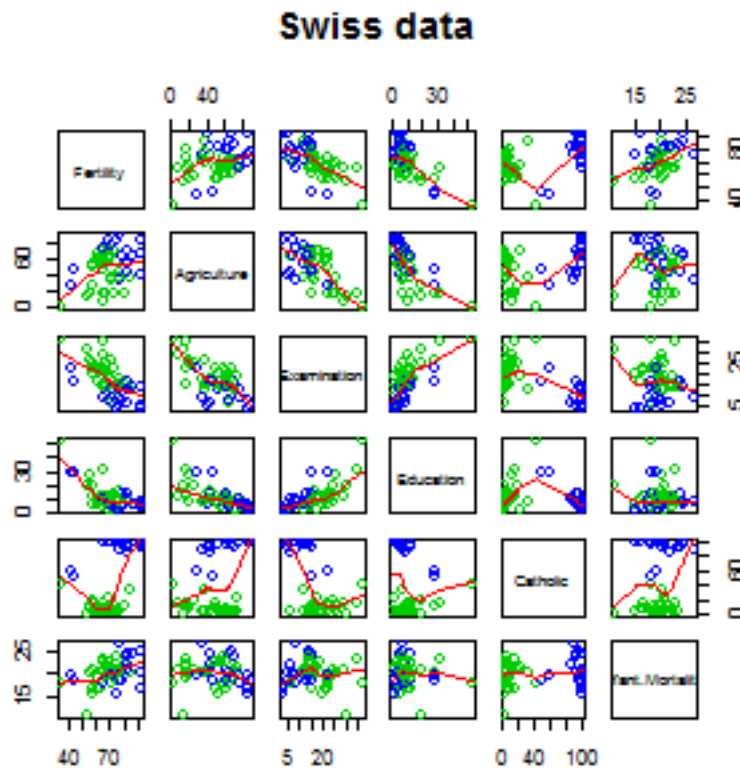
Plot of the Swiss data set
