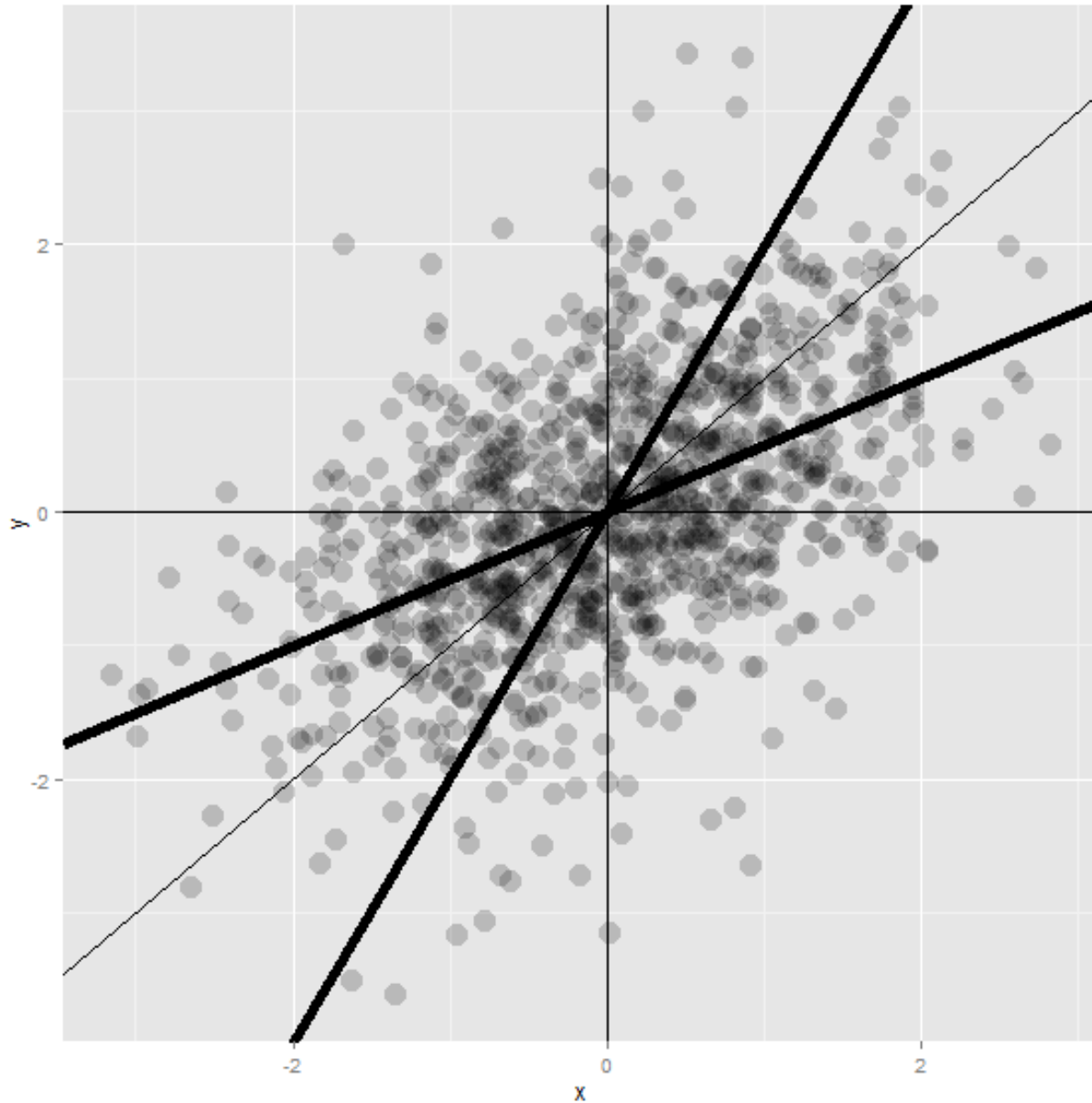
Regression to the mean, illustrated.
