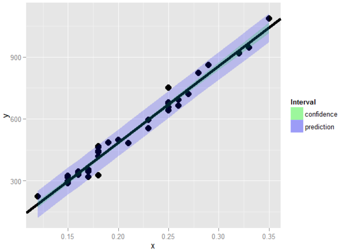
Image of prediction and mean value interval.
