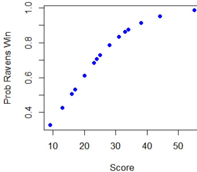
Fitted model for the Ravens data.
