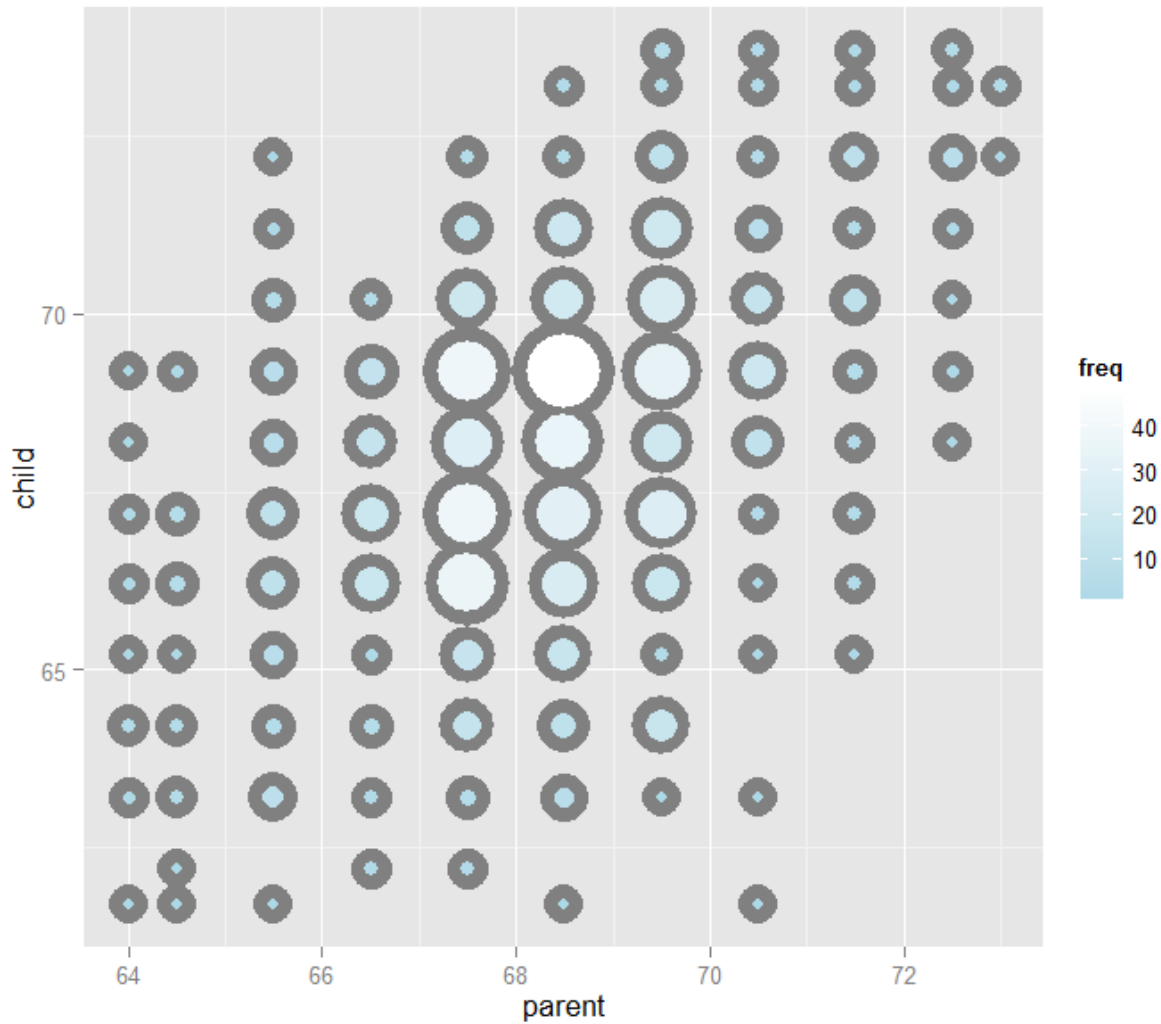
Re plot of the data
