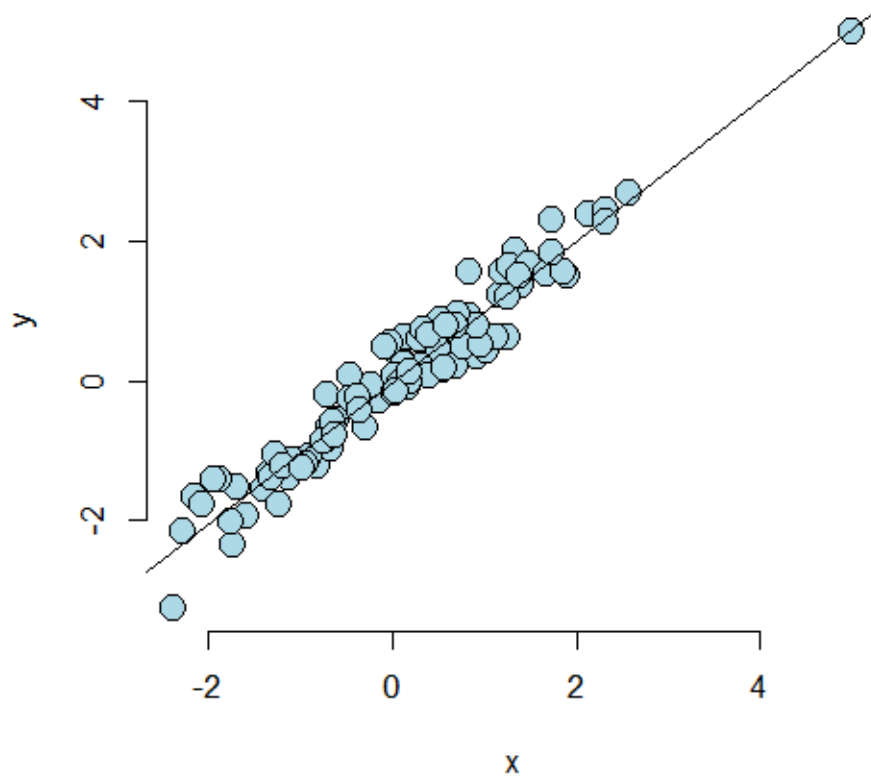
Second simulation example.
