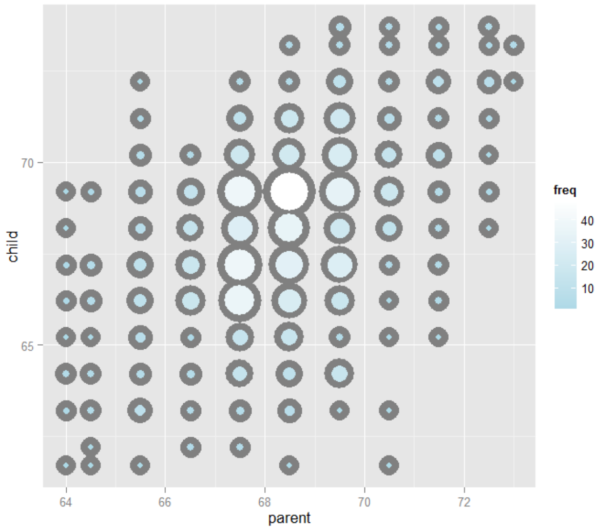
Plot of parent and child heights.
