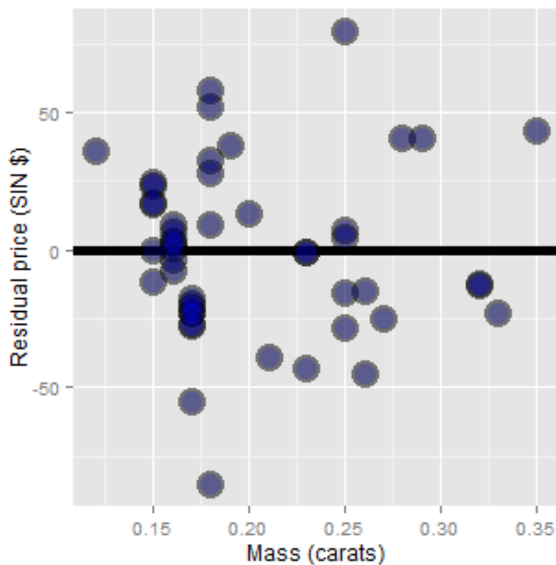
Residuals versus X.
