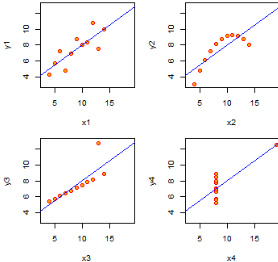
Plot of Anscombe's data set.
