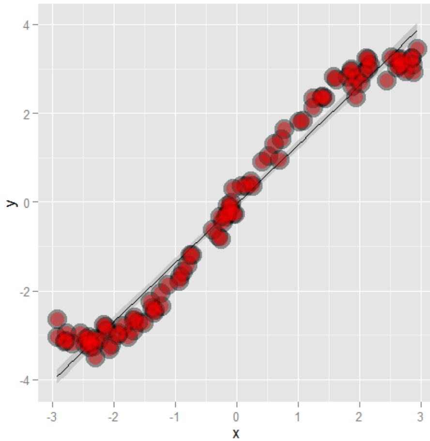
Plot of simulated non-linear data.
