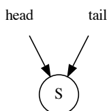
Figure 11.1: Both head and tail point to S for empty queue.
