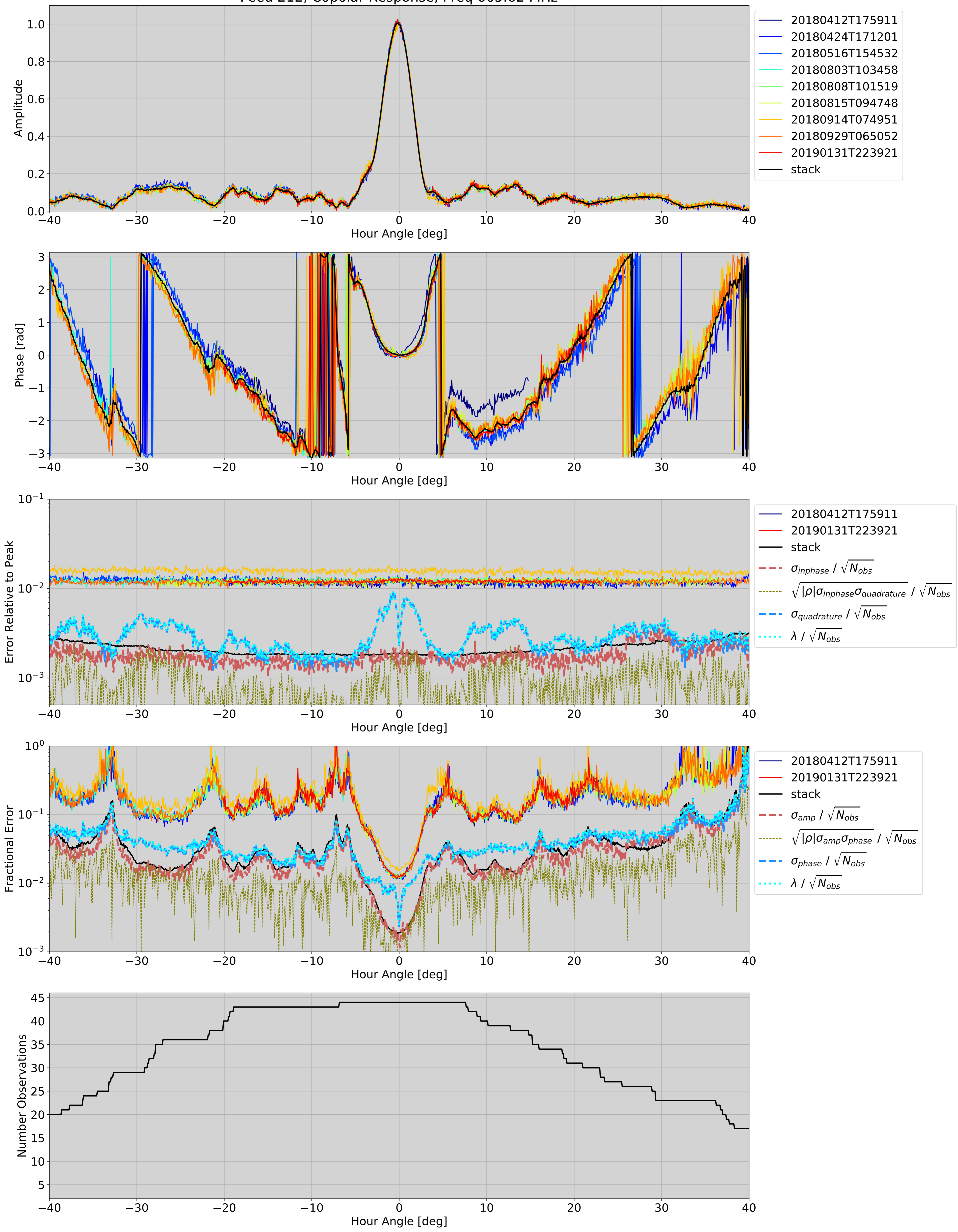
Feed 212, Copolar Response, Freq 665.62 MHz
