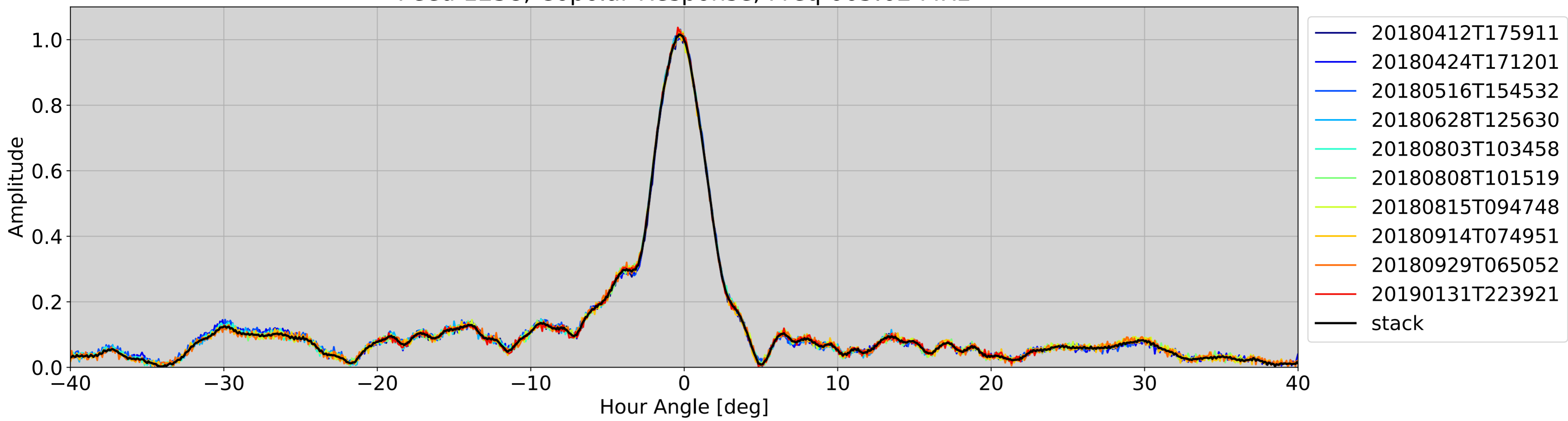
Feed 1258, Copolar Response, Freq 665.62 MHz
