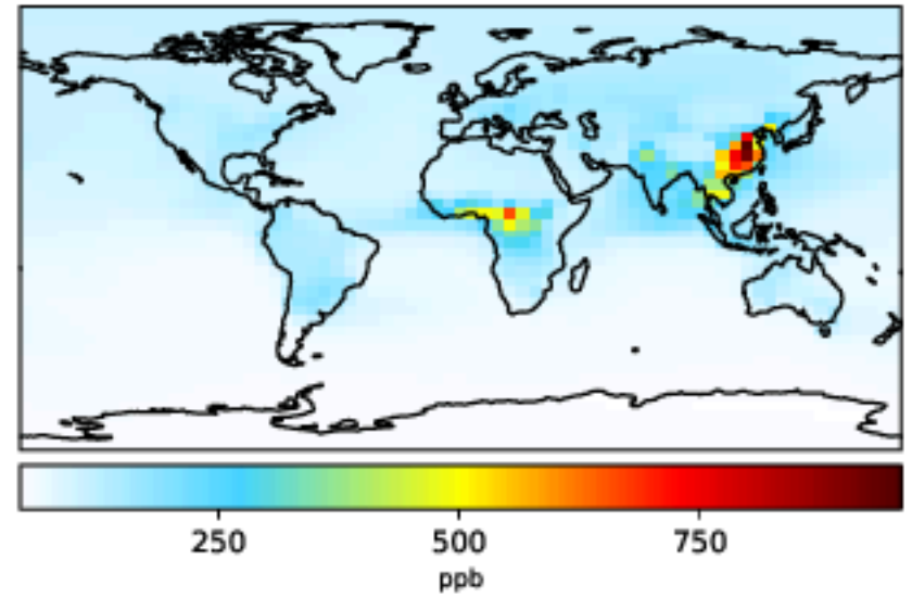
gcc_CO (Dev) 4.0x5.0
