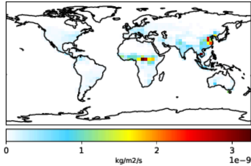
gcc_CO (Dev) 4.0x5.0
