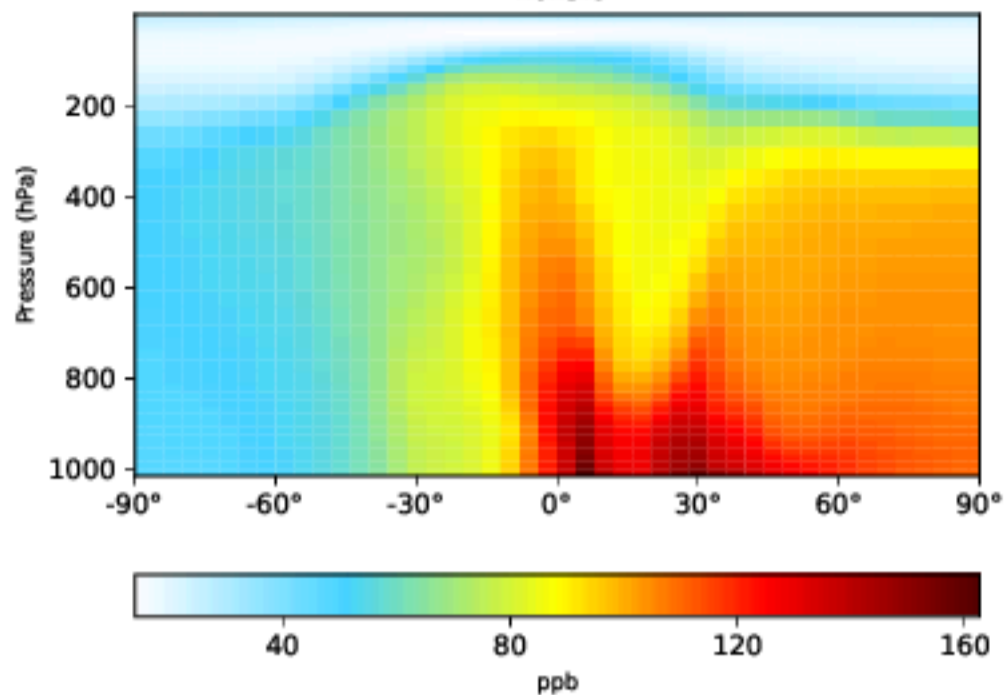
gcc_CO (Dev) 4.0x5.0
